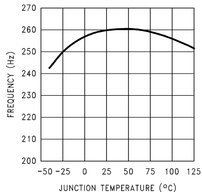
Switching Frequency
