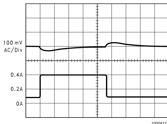
A: Output Voltage, 100 mV/div, AC-Coupled. B: Load Current: 100 mA to 400 mA Load Pulse
