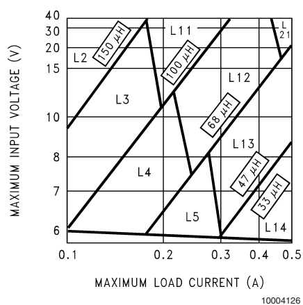
FIGURE 4. LM2674-3.3
