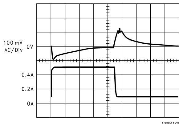
A: Output Voltage, 100 mV/div, AC-Coupled. B: Load Current: 100 mA to 500 mA Load Pulse
