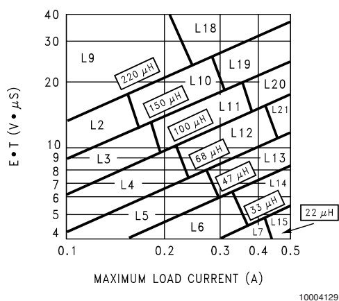
FIGURE 7. LM2674-ADJ
