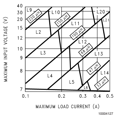
FIGURE 5. LM2674-5.0
