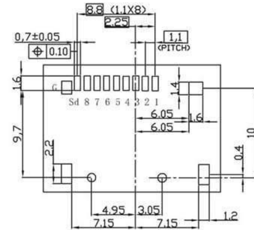
RECMMENT PC BOARD LAYOUT
